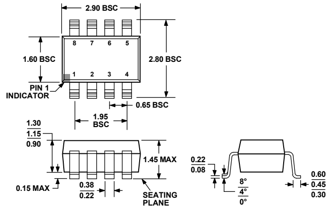
Figure 49. 8-Lead Small Outline Transistor Package [SOT-23] (RJ-8)
