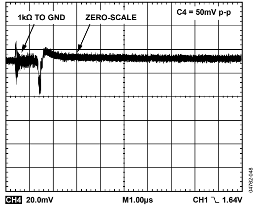
Figure 31. Typical Glitch upon Exiting Software Power-Down to Zero-Scale
