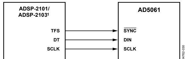
Figure 40. AD5061-to-ADSP-2101/ADSP-2103 Interface
